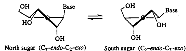
Scheme 1. Dynamic Two-State Equilibrium of N \rightleftharpoons S Pseudorotamers of \beta -D-Ribofuranosyl- C -nucleosides in Solution
