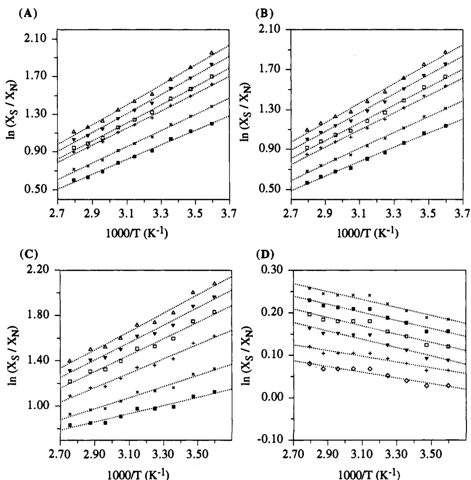
Figure 1. Van't Hoff plots of \ln(X_S/X_N) as a function of 1000/T for 1 (A), 2 (B), 3 (C), and 4 (D). The natural logarithm of the mole fractions X_S and X_N from various PSEUROT 9 analyses of temperature-dependent 3 J HH was used to perform least-squares fitting processes with PROFIT 11 to give as many straight lines as possible (see Table 2 for the conformational space covered by the PSEUROT 9 analyses). For clarity we only show representative plots based on the following PSEUROT 9 analyses: \Psi_m of both N and S conformers were constrained to 37° (+), 41° (×), and 45° (■) for 1 and 2, to 35° (+), 39° (×), and 43° (■) for 3, and to 36° (◇), 37° (+), 38° (×), 39° (■), 40° (□), and 41° (▼) for 4. P_N was also set to 0° for 1 and 2 ( \Psi_N = 37^\circ (□), 41° (▼), 45° (Δ)) and 3 ( \Psi_N = 35^\circ (□), 39° (▼), and 43° (Δ)). Individual enthalpy ( \Delta H^\circ ) and entropy ( \Delta S^\circ ) values were derived from the slopes and intercepts, respectively, of each van't Hoff plot according to the relation \ln(X_S/X_N) = -(\Delta H^\circ/R)(1000/T) + \Delta S^\circ/R and were used subsequently to calculate average \Delta H^\circ and \Delta S^\circ contributions to the N \rightleftharpoons S equilibrium of 1–4 (Table 3).
